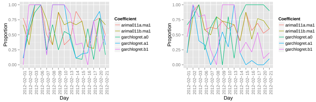
Figure 6.11: The proportion of solutions on the Pareto front for which the coefficients of the auxiliary model fit to the real data lie within the 95% confidence interval of the coefficients of the auxiliary model fit to the simulated data, for each trading day between 01/02/2012 and 21/02/2012 for 2 stocks. (Left): BNP Paribas. (Right): Credit Agricole.
